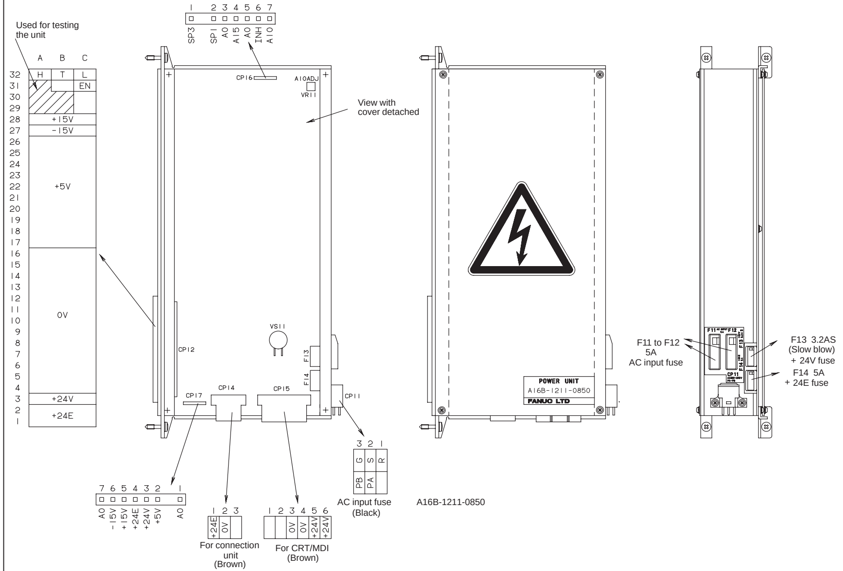
Fig.2.7.1(a) Power supply unit A external diagram
